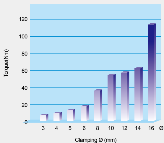
20mm dia. Chuck with Sleeves
