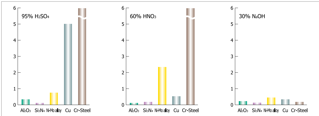
CORROSION RESISTANCE (mg/cm 3 , boiling, 30min.)
