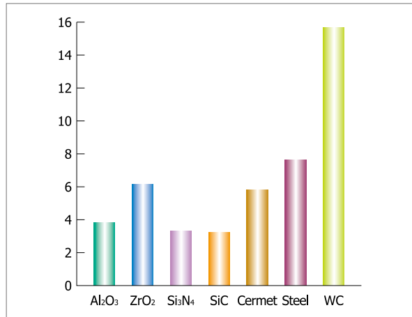
DENSITY (g/cm 3 )
