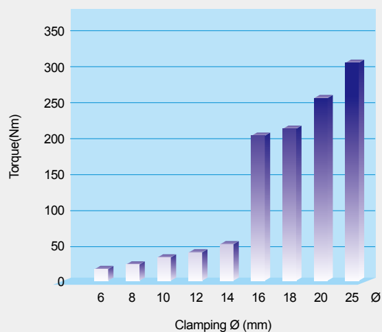
32mm dia. Chuck with Sleeves
