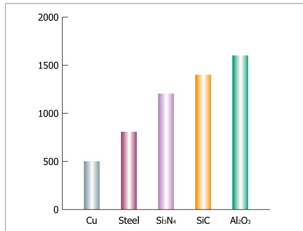
WORKING TEMP. (°C, in air)
